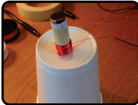
Step 5: Punch hole in bottom of cup and insert paper tube with magnet and coil
