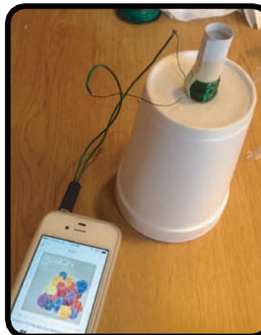
Step 8: Plug audio jack into phone or computer and play!
