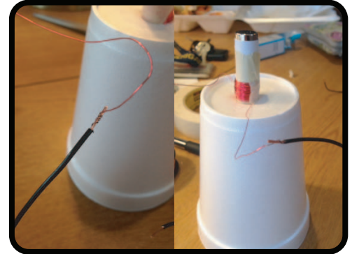
Step 6: Connect magnet wire with audio jack
